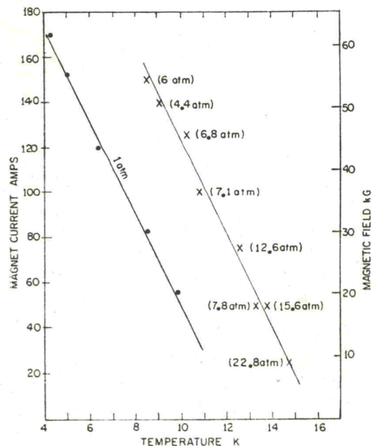
FIG. 1. Quench current vs temperature for Nb 3 Sn ribbon solenoid. ●—Points taken at atmospheric pressure, ×—points at the elevated pressure given.
